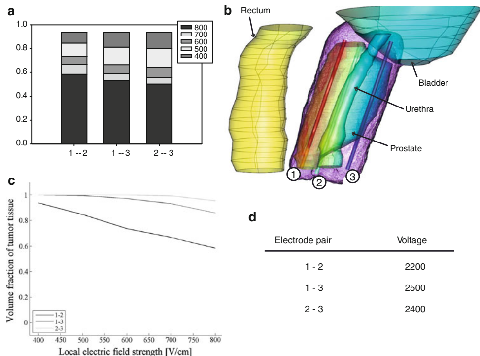
Fig. 4 Excerpt from a prepared treatment plan for N-TIRE of prostate cancer. a Electrode pair contribution, b model with three needle electrodes, c cumulative coverage curves showing that the whole tumor is covered with fields in excess of 700 V/cm and >95 % of the tumor is covered with fields in excess of 800 V/cm, d voltages used in the proposed treatment plan
